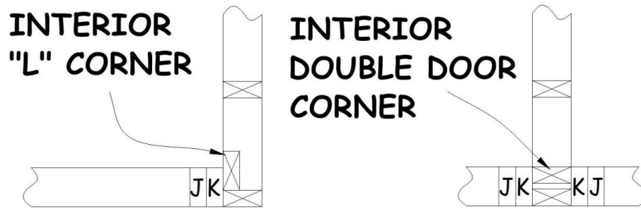
Figure 6-6. Corner Construction.
