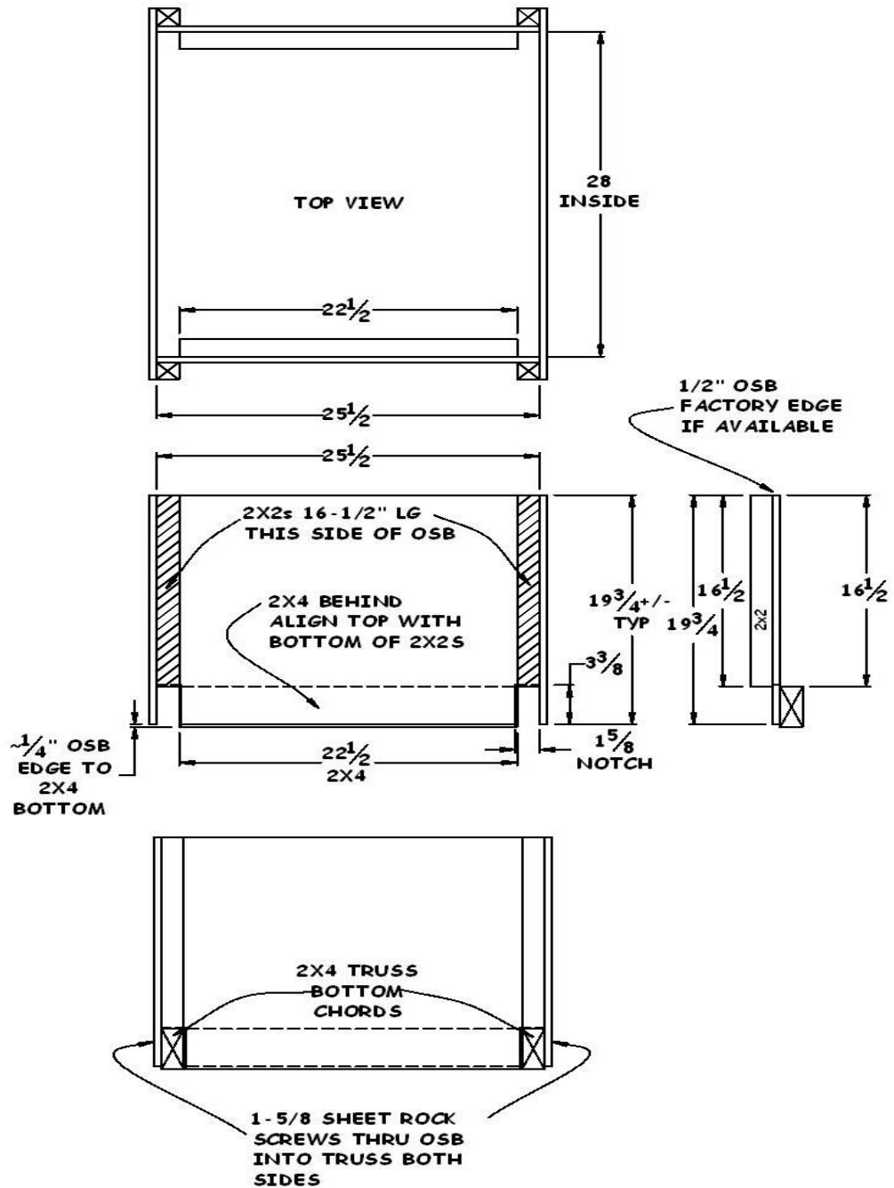
Figure 7-5. Scuttle Box Assembly.
