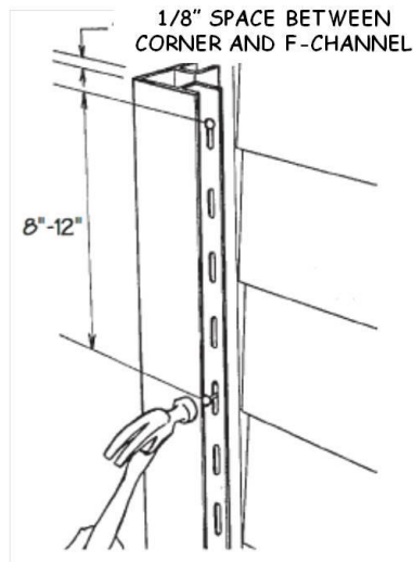
Figure 11-2. Siding Corner Post .
