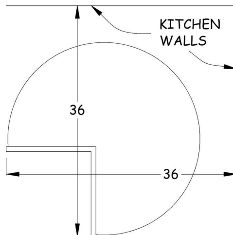
Figure 17-1. Corner Cabinet Installation
