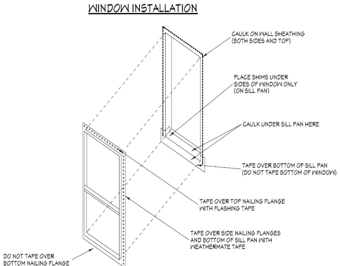
Figure 9-1. Window Installation
