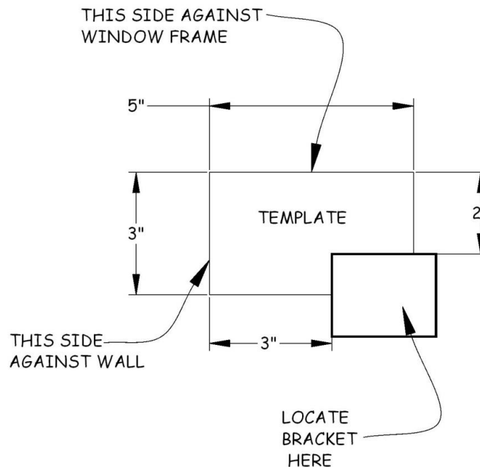
Figure 19-6. Miniblind Installation Guide.
