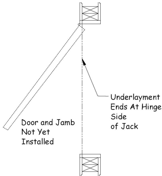
Figure 16-1. Underlayment in Interior Door Opening.
