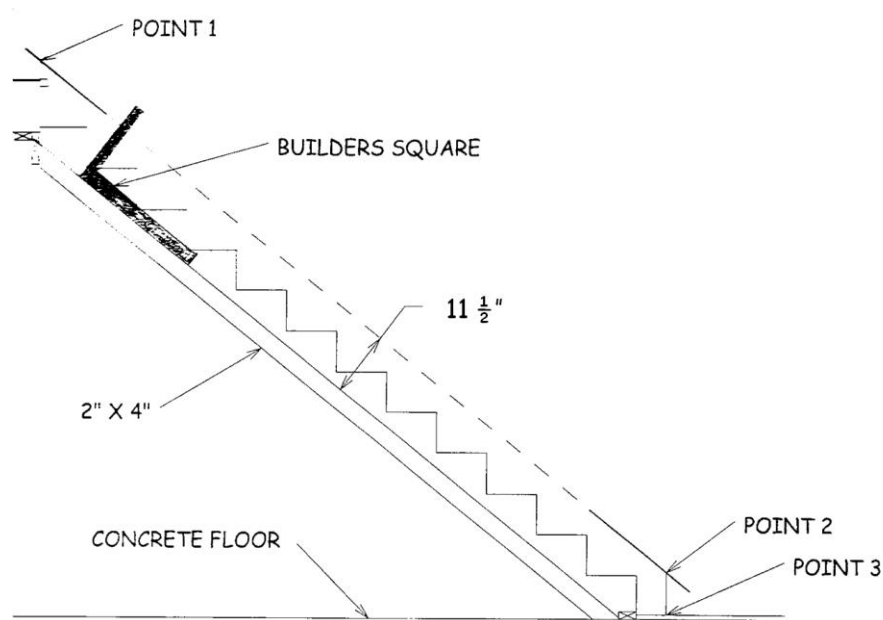
Figure 16-3. Skirtboard Installation.
