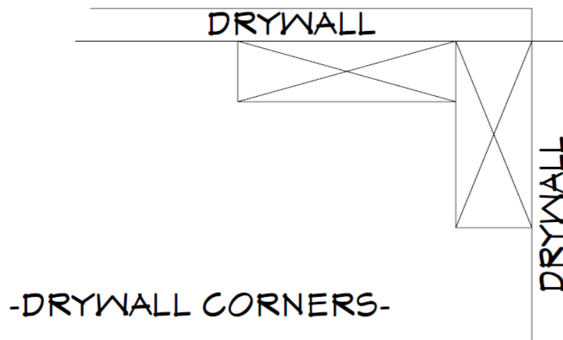
Figure 14-1. Outside Corner Installation of Sheetrock.
