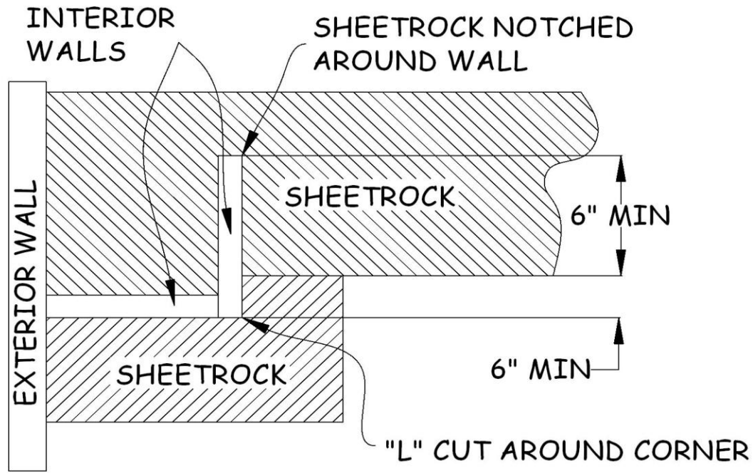
Figure 13-2. "L" and Notch Cuts Around Interior Walls
