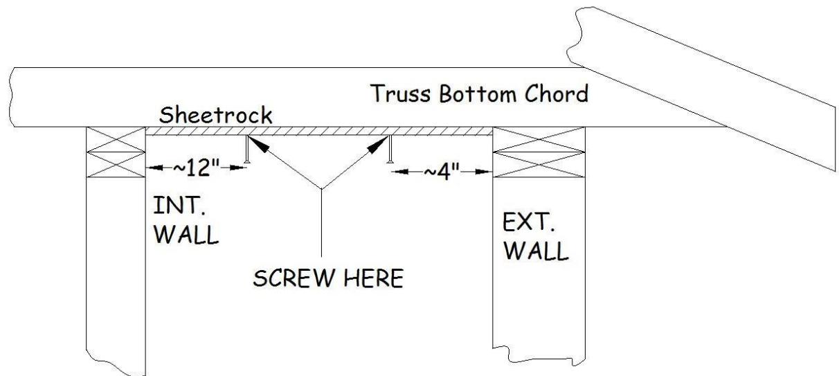
Figure 13-1. Screw Locations for Ceiling Sheetrock.
