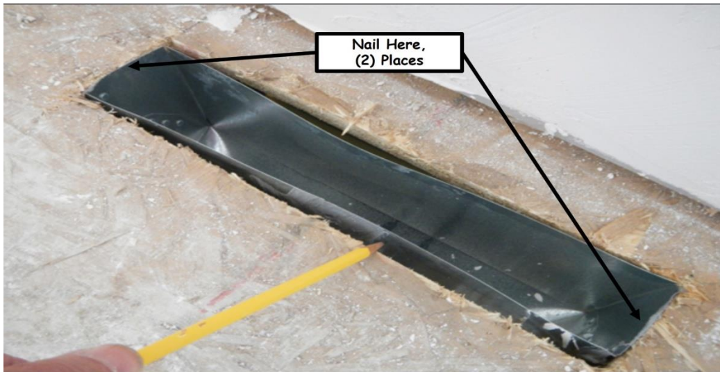
Figure 12-1. Securing In-Floor Heating Ducts
