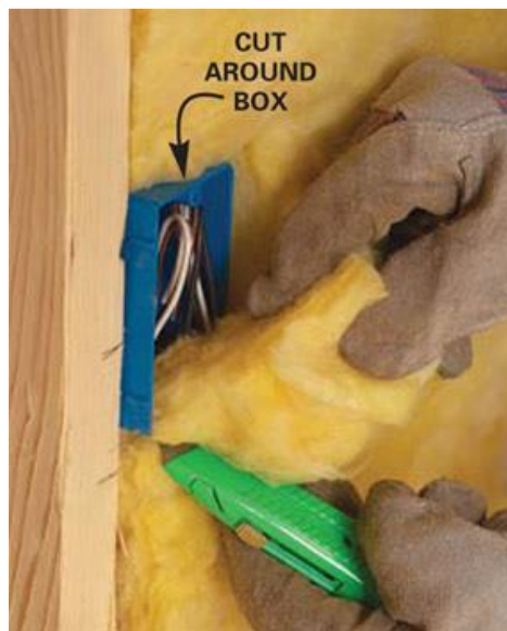
Figure 12-5. Insulating Around Electrical Box.
