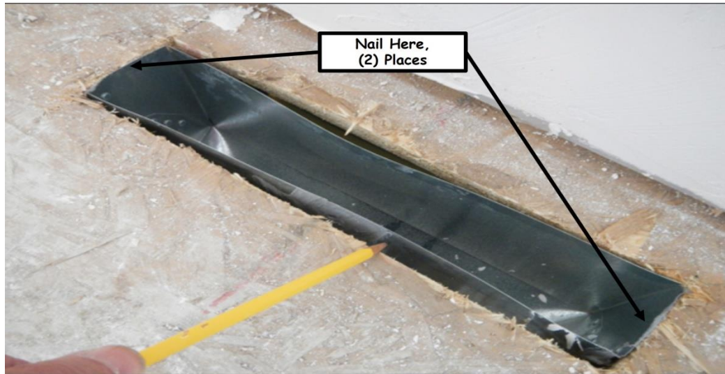
Figure 12-3. Securing In-Floor Heating Ducts
